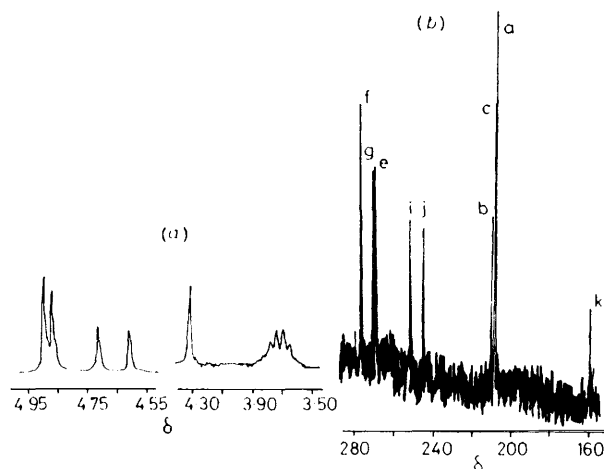
FIGURE 1 Proton (a) and 13 C (b) n.m.r. spectra of (2a) in CD 2 Cl 2 at -20 °C
