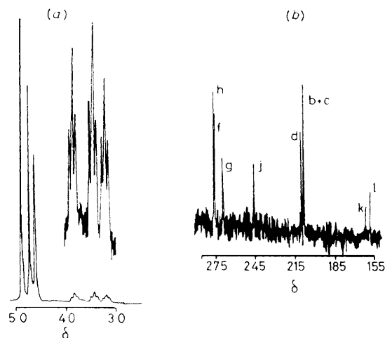
FIGURE 2 Proton (a) and ^{13}\text{C} (b) n.m.r. spectra of (2b) in \text{CD}_2\text{Cl}_2 at -20^\circ\text{C}
